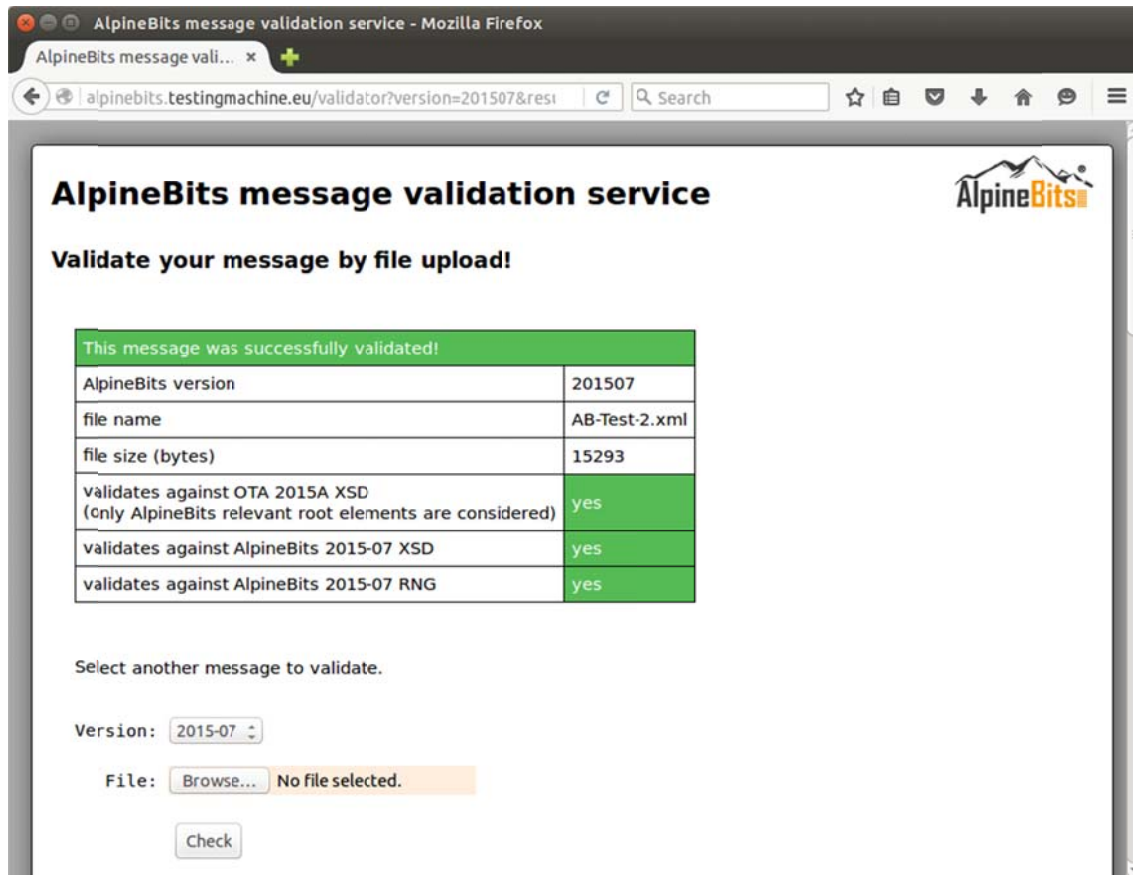
Figure 7. Validation of Output from JSON-LD Serialization
