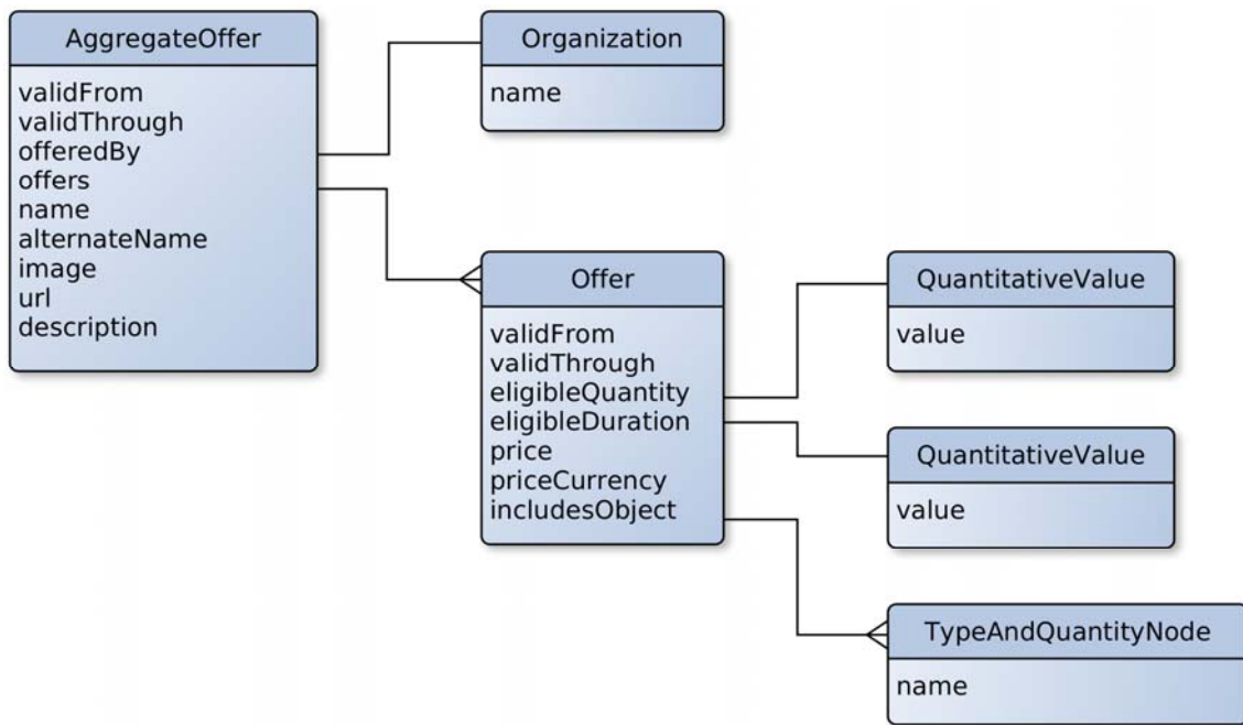
Figure 1. Classes and Properties of Schema.org obtained from the Mapping
