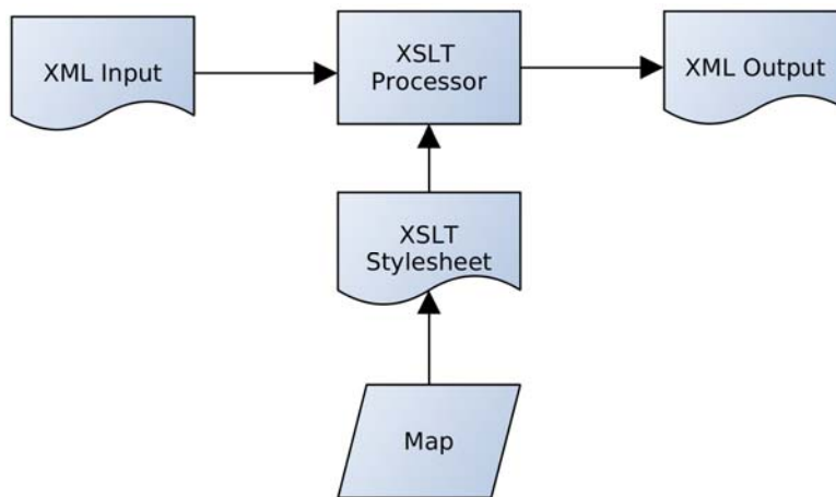
Figure 2. Implementation with XSL Transformations
